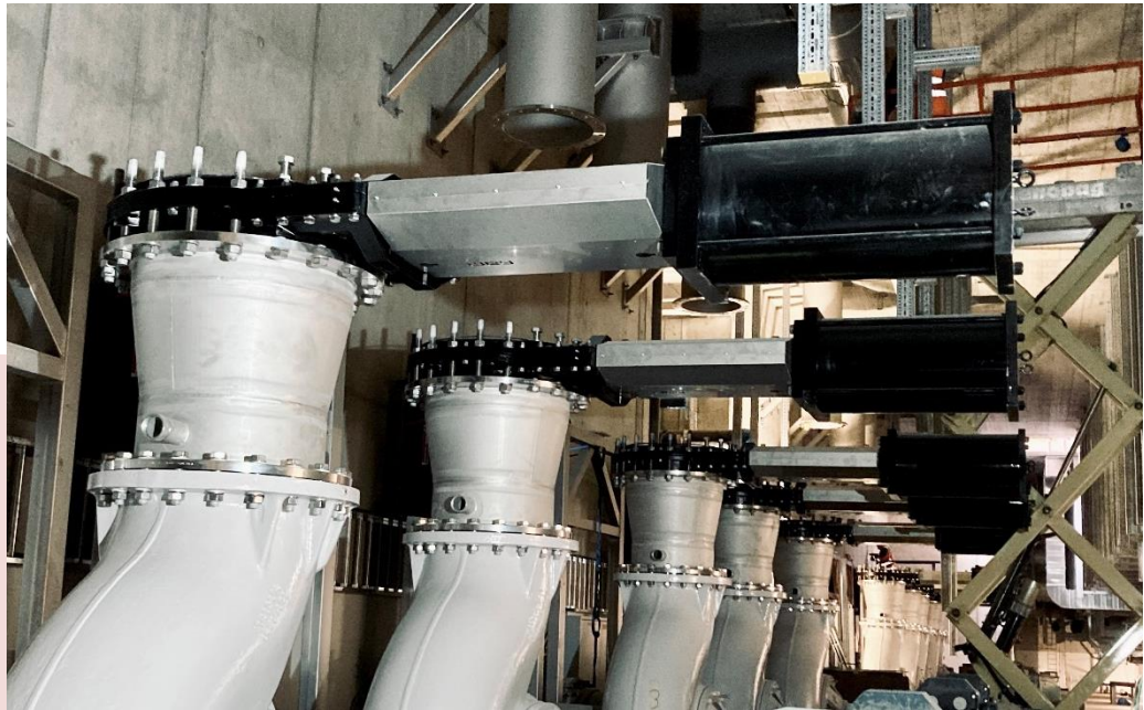
Wey MFC DN 700 knife gate valves in the biological treatment unit
